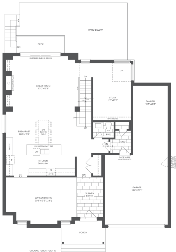
GROUND FLOOR PLAN X
